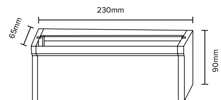
Nicho / Recessed
