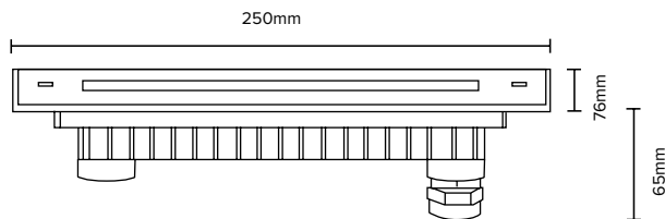
Luminaria / Spotlight
